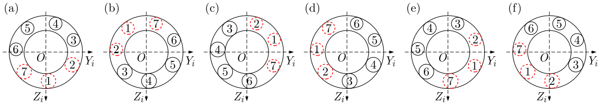
Fig. 4. Different bearing conditions
