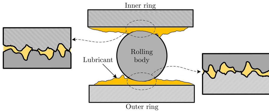
Fig. 3. Schematic of the contact surface between the RB and the raceway
