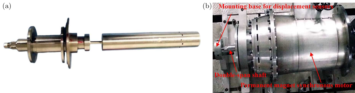
Fig. 14. Experimental device for the high-speed shaft with double spans and multiple supports: (a) double-span multi-support shaft, (b) experimental setup for the shaft
