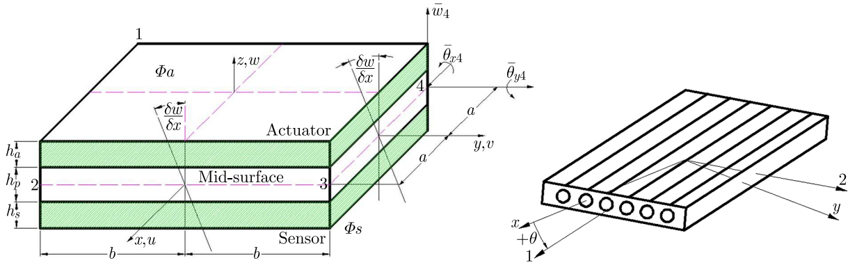
Fig. 1. A laminated finite element coordinate system with the integrated piezoelectric material (left) and the fiber direction in local and global coordinate systems (right)
