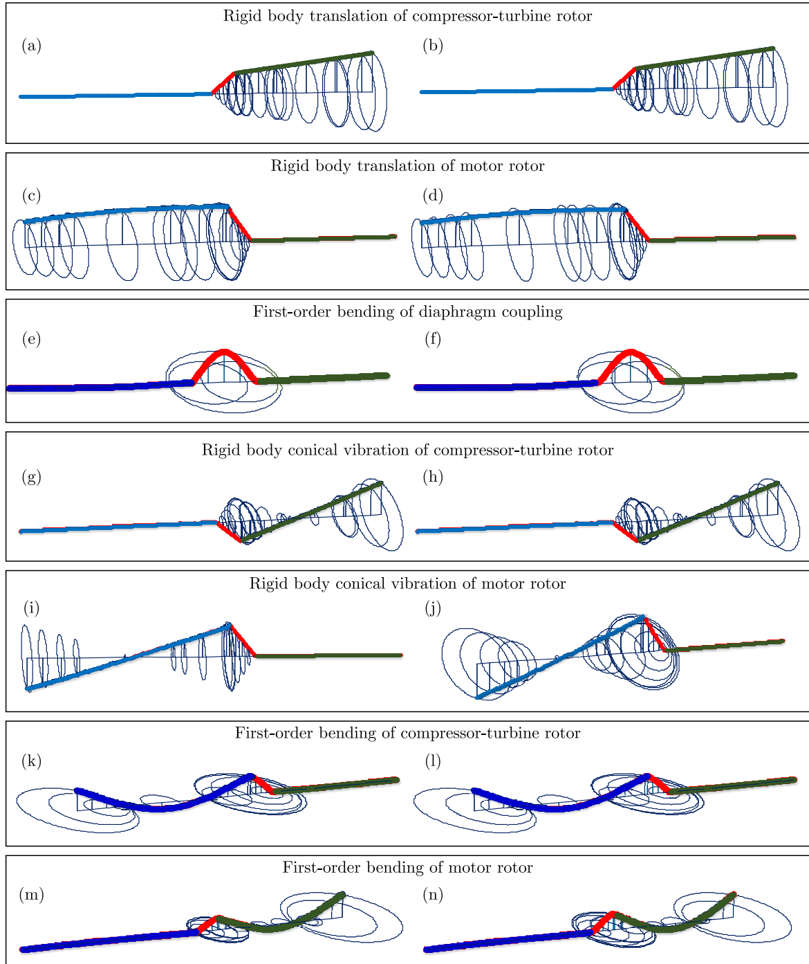
Fig. 7. Vibration mode of the double-span combined rotor shaft system
