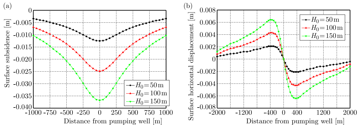
Fig. 9. Relationship between thicknesses, surface movement, and deformation
