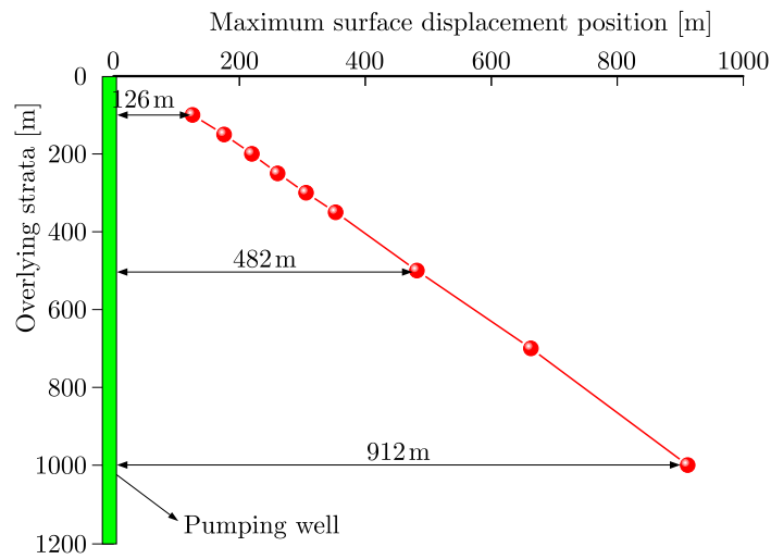
Fig. 11. Relationship between the maximum surface horizontal displacement position and overlying strata thickness
