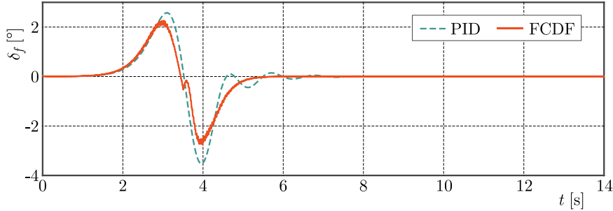
Fig. 7. Active steering angle under lane change condition
