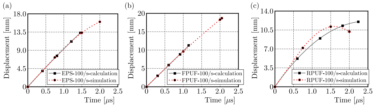
Fig. 7. Displacement-time curve comparison of the protected product by theoretical analysis and simulation: (a) EPS, (b) FPUF, (c) RPUF
