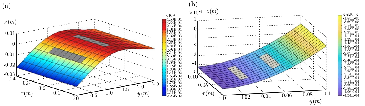
Fig. 22. The displacement of a controlled diving board in scenario 2: fiber direction [75, -75] s (left), fiber direction [30, 60] s (right)
