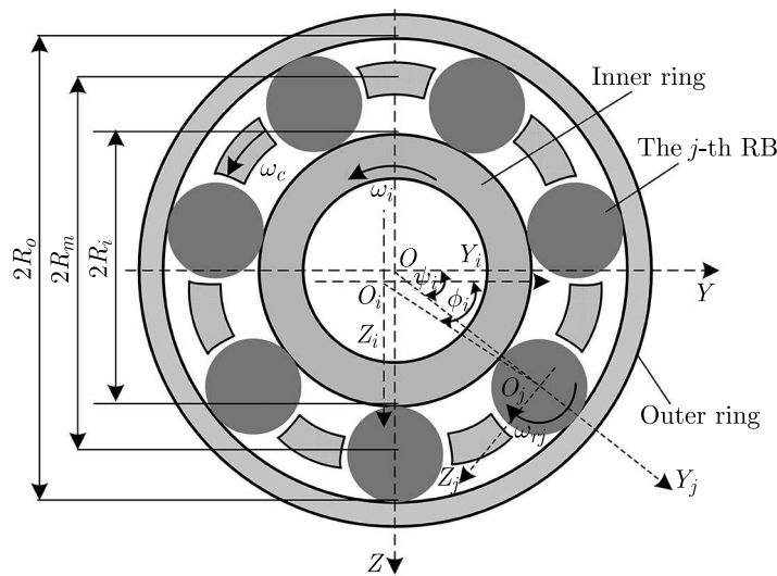
Fig. 1. Schematic of the rolling bearing
