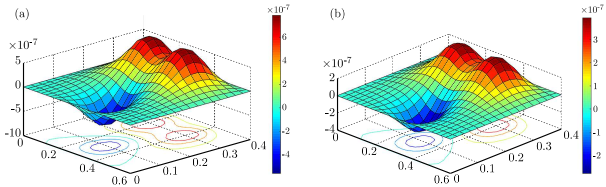
Fig. 9. The total displacement amplitude of the plate: (a) without control, (b) with control
