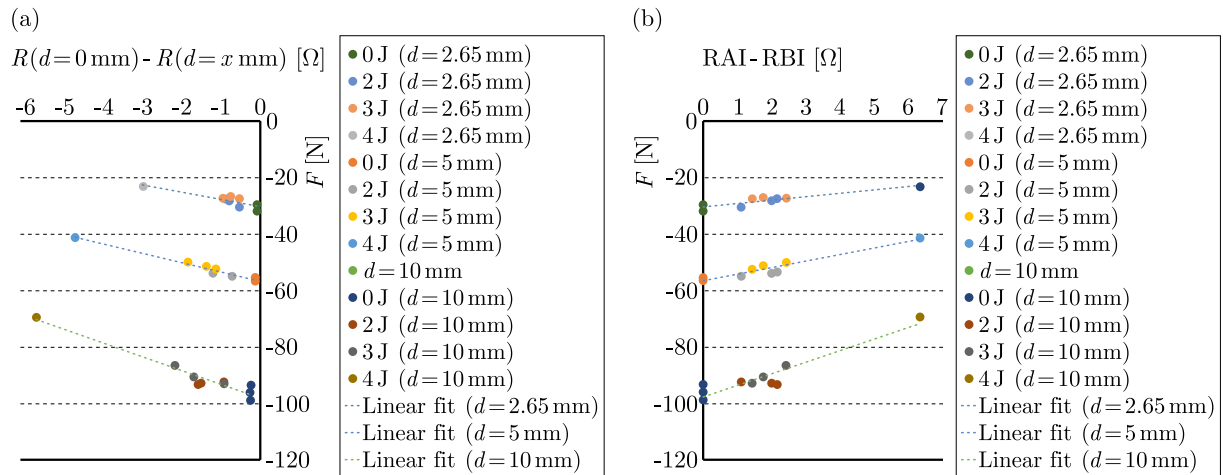
Fig. 9. Graph of force – change of measured electrical resistance for different impact energies and displacements (a) during loading ( d = x \text{ mm} ); (b) AI and BI.
