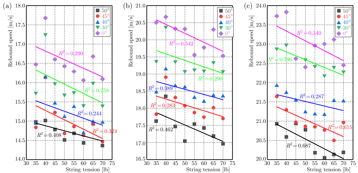
Fig. 4. Linear fitting plots of racket string tension versus rebound speed at various incidence angles and ball speeds: (a) incident speed of 20 m/s; (b) incident speed of 25 m/s; (c) incident speed of 30 m/s.
