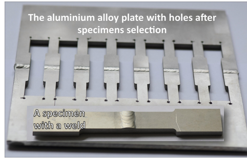
Fig. 4. Aluminium alloy plate after specimens manufacturing for examination of mechanical resistance of the weld.
