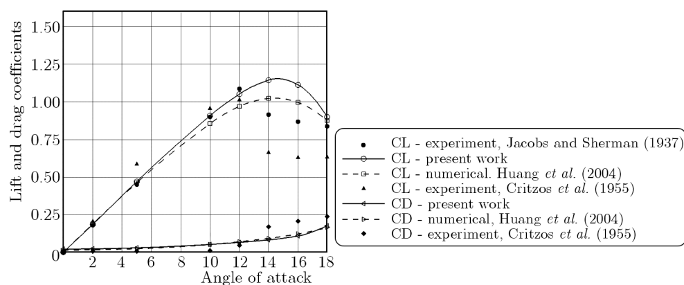
Fig. 5. Comparison between computation results with the numerical work by Huang et al. (2004) and experimental results by Critzos et al. (1955) and Jacobs and Sherman (1937)
